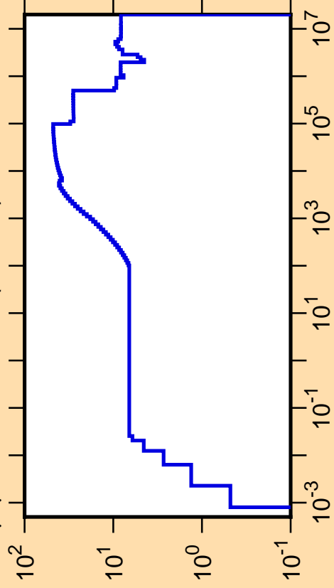
\Delta\mu/\mu vs. E for ^{110}\text{In}(\text{mt251})
