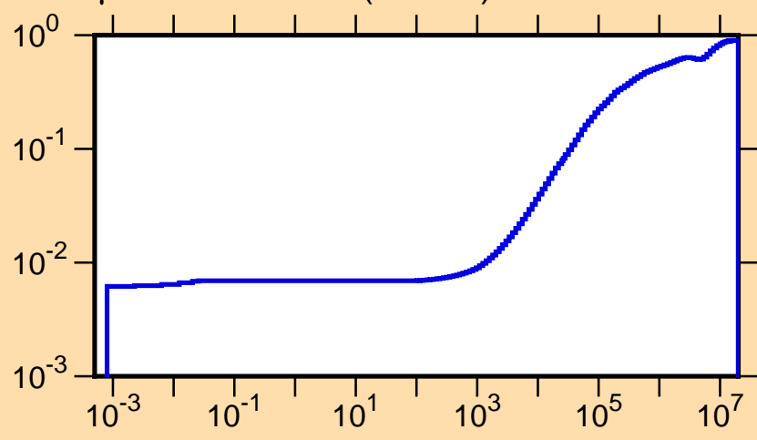
\mu vs. E for ^{110}\text{In}(\text{mt251})
