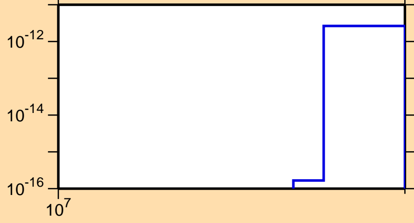
\sigma vs. E for ^{110}\text{In} (mt 34)
