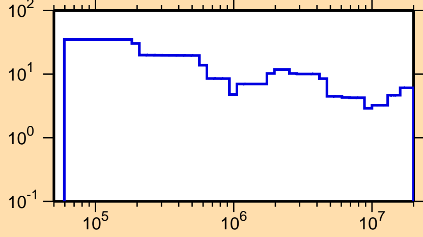
\Delta\sigma/\sigma vs. E for ^{110}\text{In}(n,\text{tot.})
