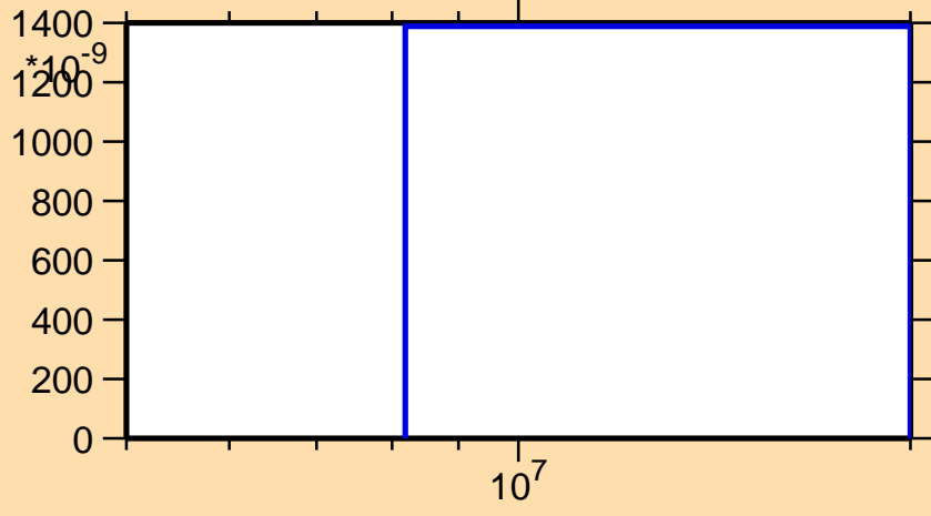
\sigma vs. E for ^{110}\text{In}(n,nd)
