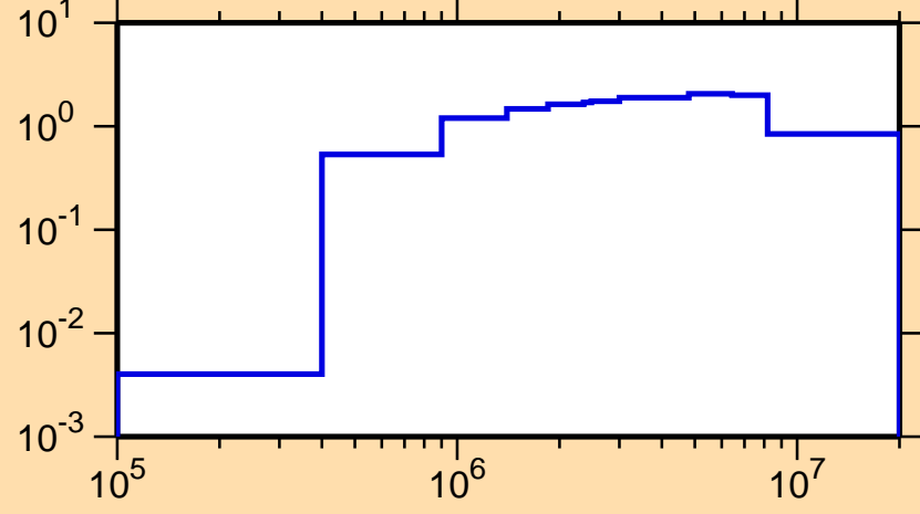
\sigma vs. E for ^{110}\text{In}(n,\text{inel.})
