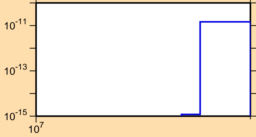
\sigma vs. E for ^{110}\text{In}(n,\text{pt})
