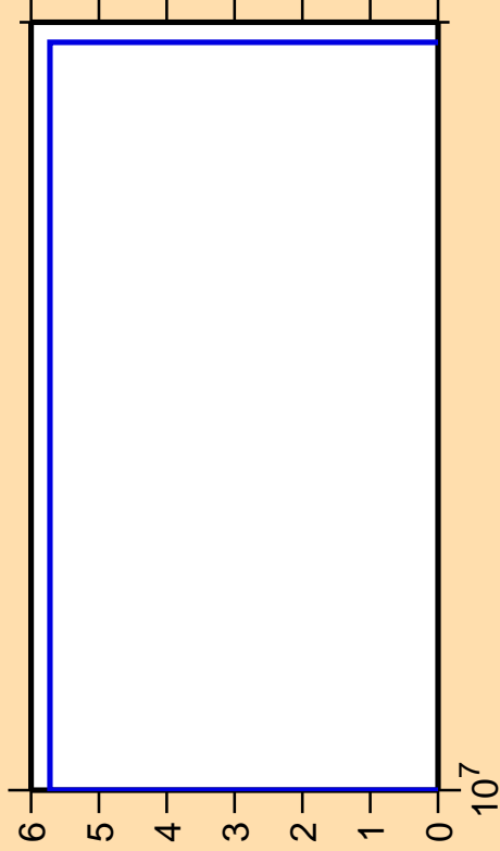
\Delta\sigma/\sigma vs. E for ^{110}\text{In} (mt 45)
