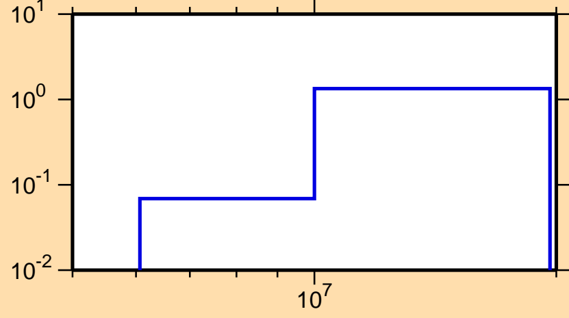
\sigma vs. E for ^{110}\text{In}(n,2n)
