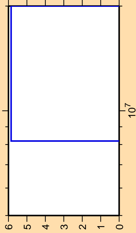
\Delta\sigma/\sigma vs. E for ^{110}\text{In}(\text{mt } 45)
