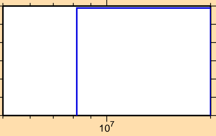
\sigma vs. E for ^{110}\text{In}(\text{mt } 45)
