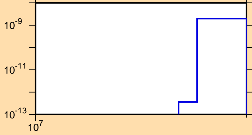
\sigma vs. E for ^{111}\text{In}(n,2n\alpha)
