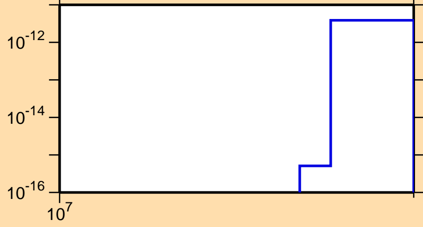
\sigma vs. E for ^{111}\text{In}(n,\text{pd})
