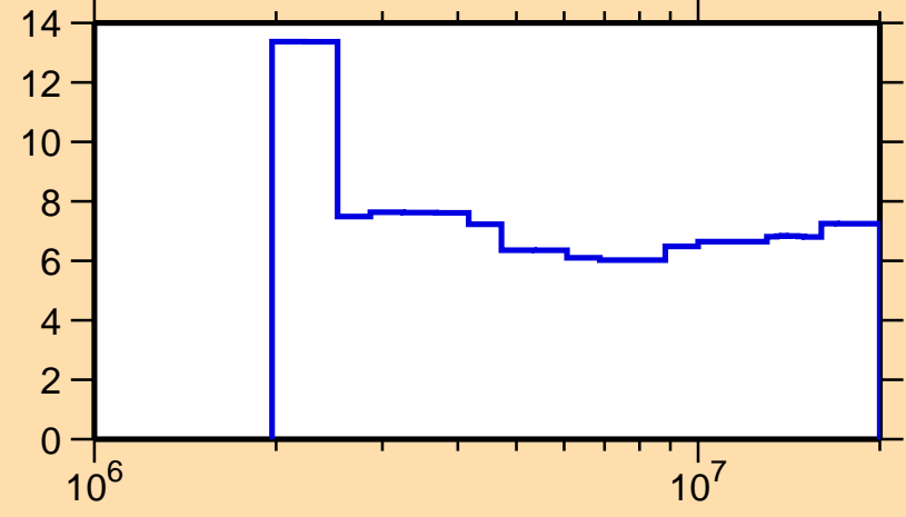
\Delta\sigma/\sigma vs. E for ^{111}\text{In}(n,n\text{nonel.})
