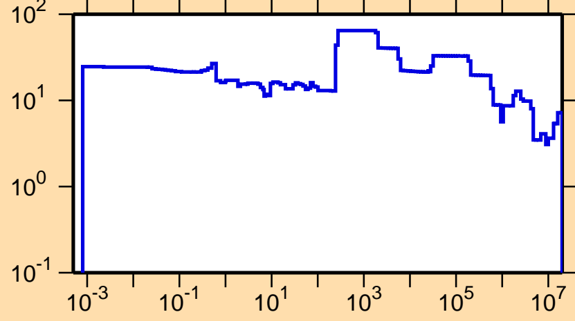
\Delta\sigma/\sigma vs. E for ^{111}\text{In}(n,\text{tot.})
