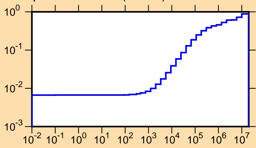
\mu vs. E for ^{111}\text{In}(\text{mt251})
