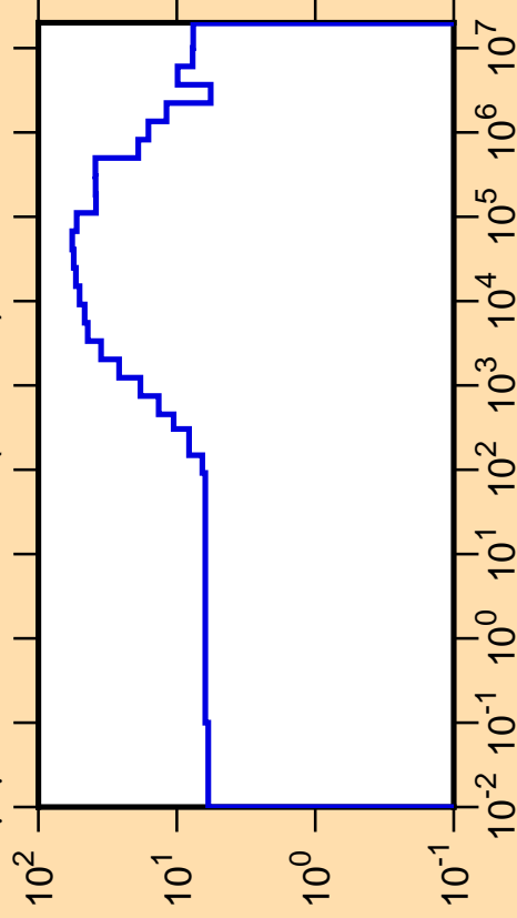
\Delta\mu/\mu vs. E for ^{111}\text{In}(\text{mt251})
