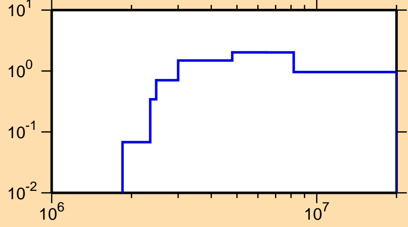
\sigma vs. E for ^{111}\text{In}(n,n\text{cont.})
