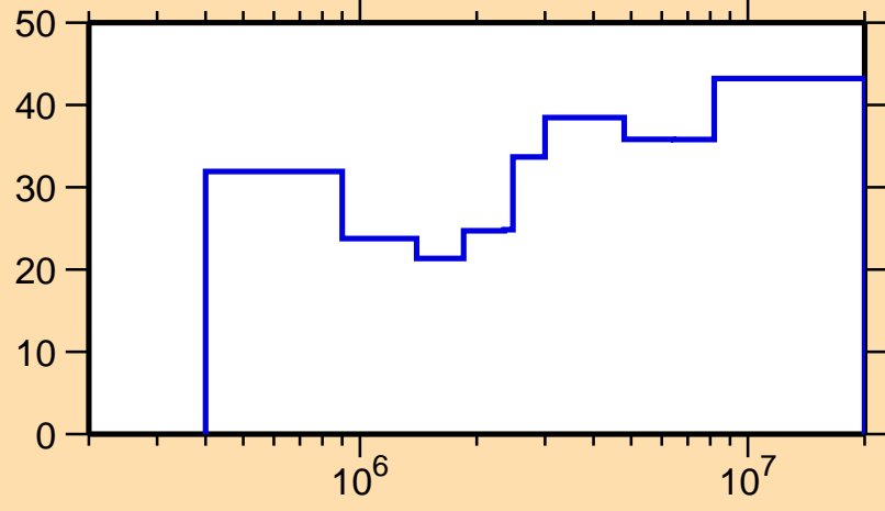
\Delta\sigma/\sigma vs. E for ^{111}\text{In}(n,n_1)
