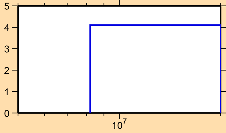
\Delta\sigma/\sigma vs. E for ^{111}\text{In}(n,\text{tot.})
