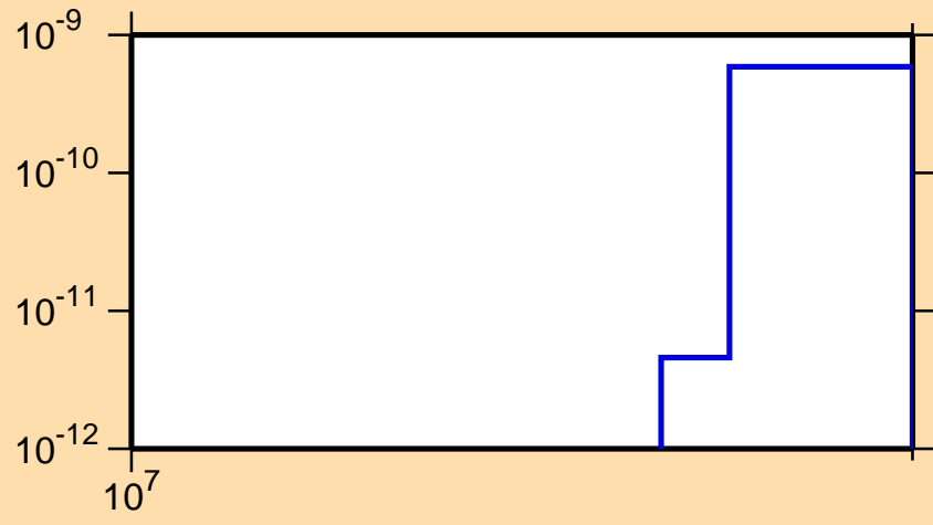
\sigma vs. E for ^{111}\text{In} (mt 45)
