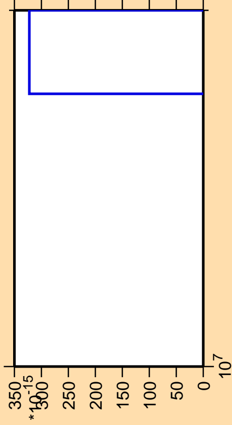
\Delta\sigma/\sigma vs. E for ^{111}\text{In} (mt 11)
