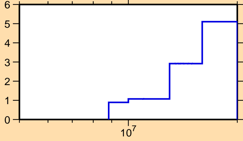
\Delta\sigma/\sigma vs. E for ^{111}\text{In}(n,\text{el.})
