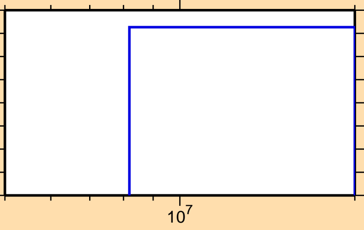
\sigma vs. E for ^{111}\text{In}(n,\text{He3})
