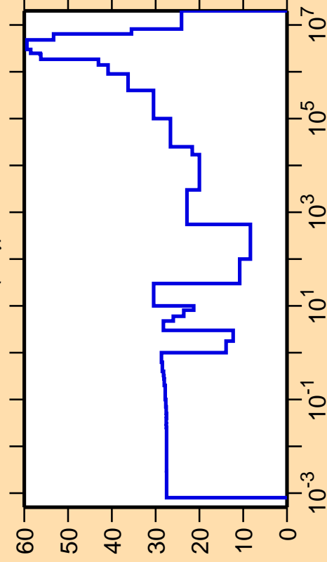
\Delta\sigma/\sigma vs. E for ^{111}\text{In}(n,\gamma)
