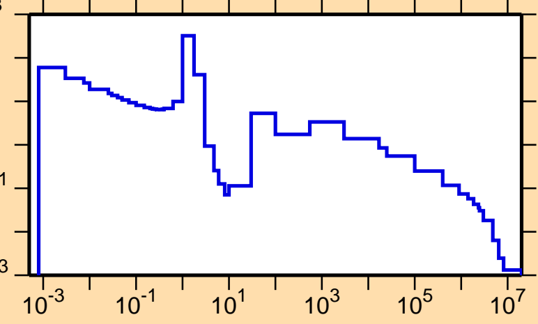
\sigma vs. E for ^{111}\text{In}(n,\gamma)
