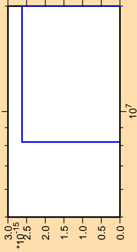
\Delta\sigma/\sigma vs. E for ^{111}\text{In}(\text{mt } 11)
