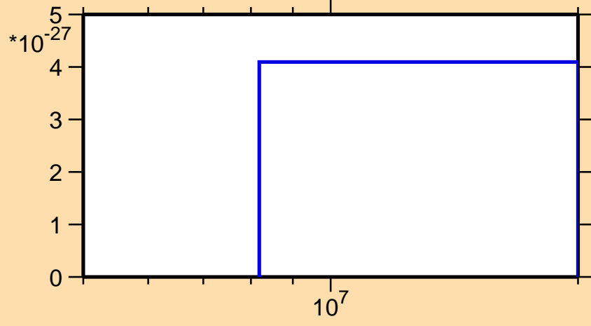
\sigma vs. E for ^{111}\text{In}(\text{mt } 11)
