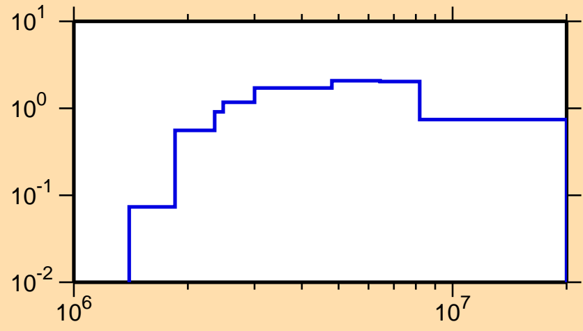
\sigma vs. E for ^{111}\text{In}(n,n\text{cont.})
