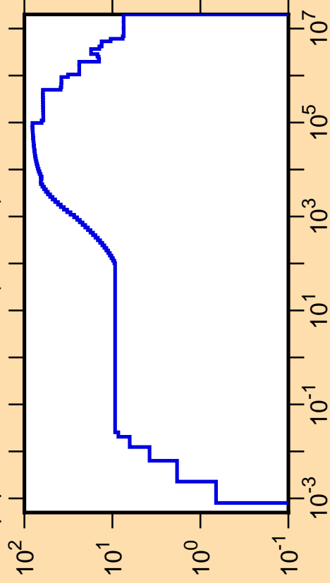
\Delta\mu/\mu vs. E for ^{112}\text{In}(\text{mt251})
