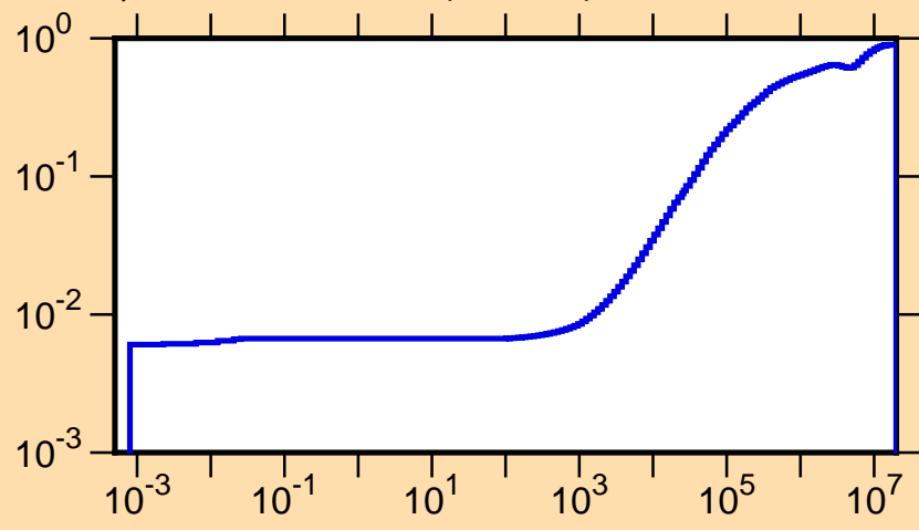
\mu vs. E for ^{112}\text{In}(\text{mt251})
