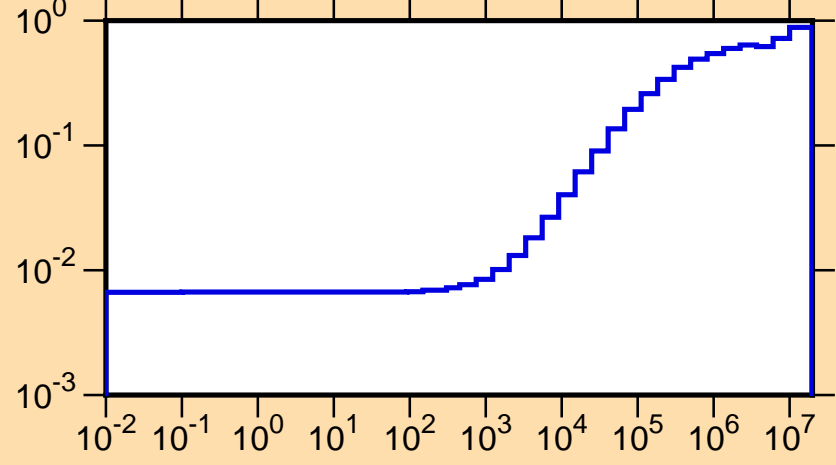
\mu vs. E for ^{112}\text{In}(\text{mt251})
