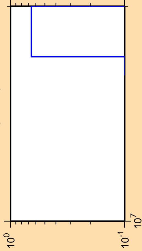
\Delta\sigma/\sigma vs. E for ^{112}\text{In} (mt 45)
