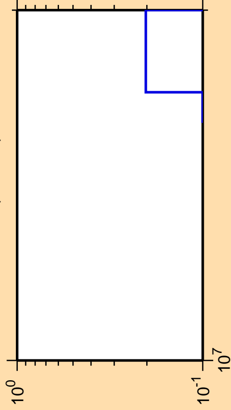
\Delta\sigma/\sigma vs. E for ^{112}\text{In}(\text{mt117})
