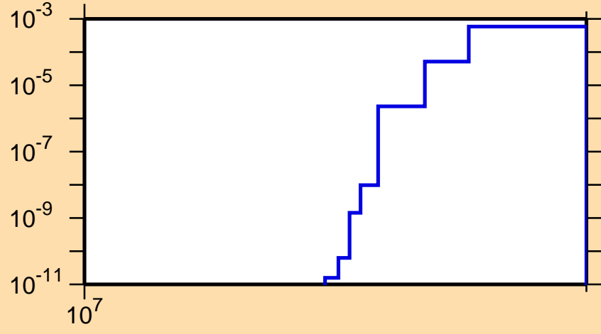
\sigma vs. E for ^{112}\text{In}(n,2np)
