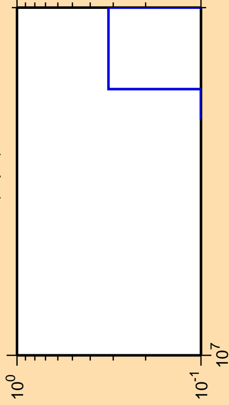
\Delta\sigma/\sigma vs. E for ^{112}\text{In}(n,\text{pd})
