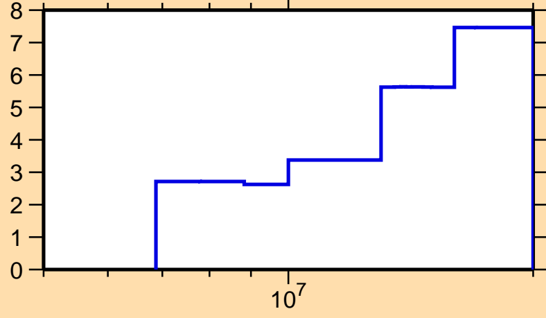
\Delta\sigma/\sigma vs. E for ^{112}\text{In}(n,\text{tot.})
