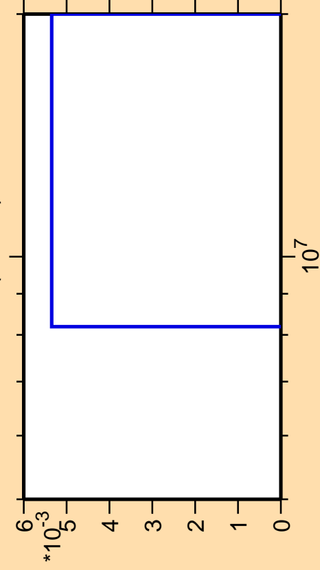
\Delta\sigma/\sigma vs. E for ^{112}\text{In}(\text{mt } 45)
