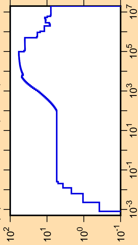
\Delta\mu/\mu vs. E for ^{113}\text{In}(\text{mt251})
