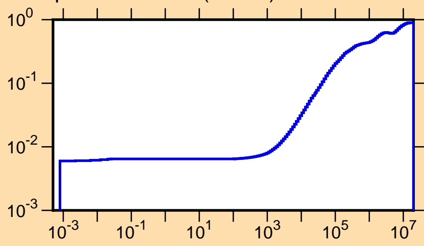
\mu vs. E for ^{113}\text{In}(\text{mt251})
