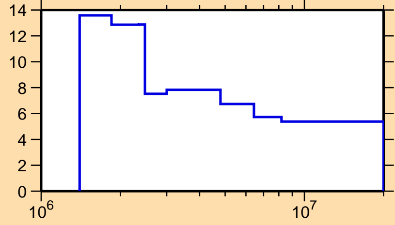
\Delta\sigma/\sigma vs. E for ^{113}\text{In}(n,n\text{nonel.})
