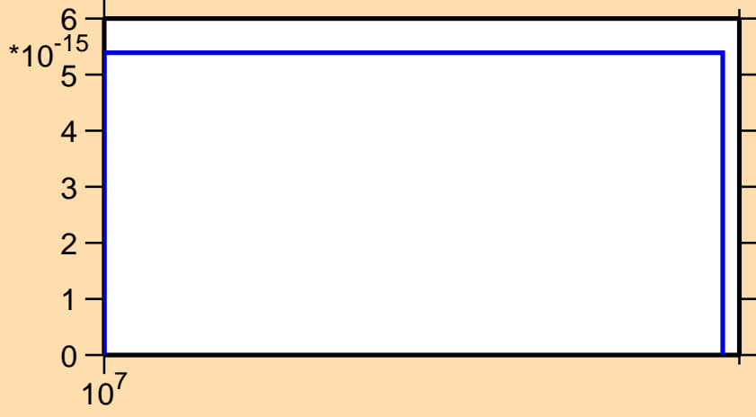
\sigma vs. E for ^{113}\text{In} (mt 45)
