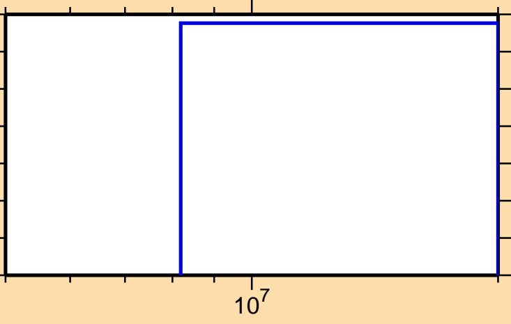
\sigma vs. E for ^{113}\text{In}(n,3n)
