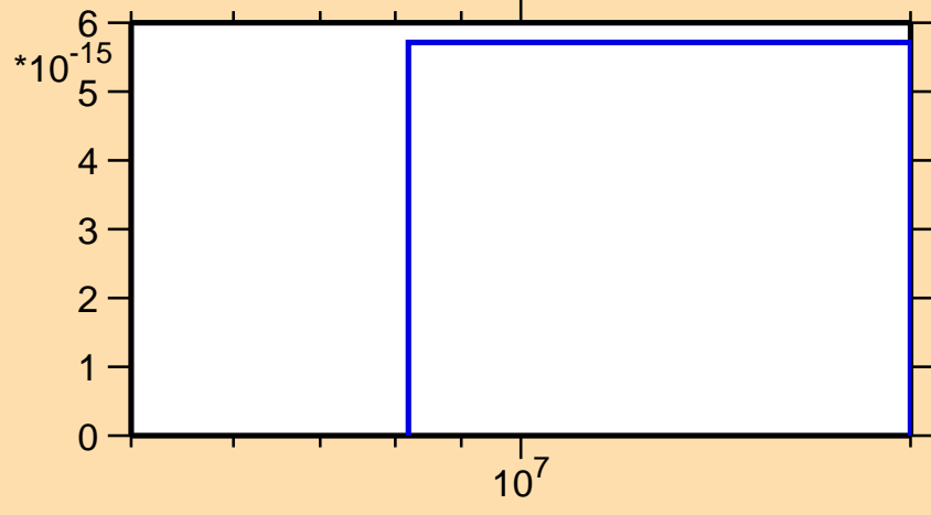
\sigma vs. E for ^{113}\text{In}(\text{mt } 45)
