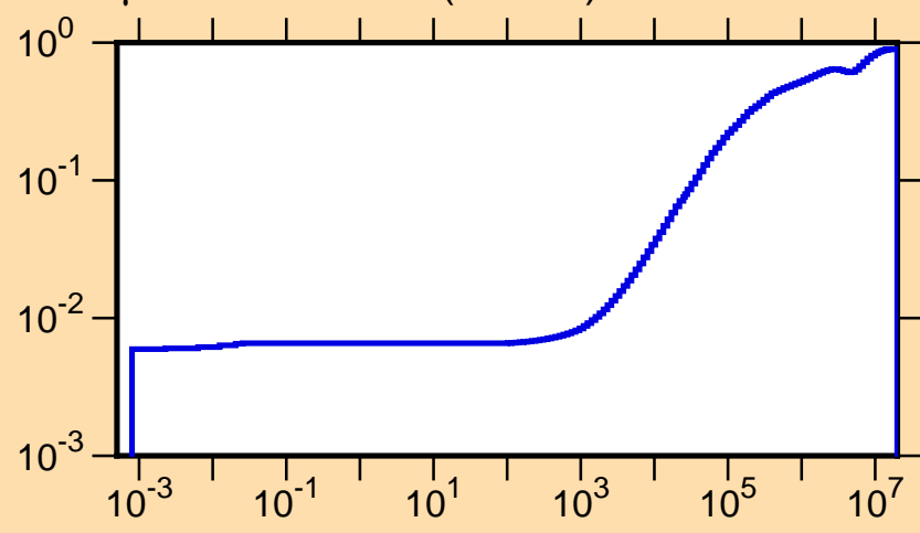
\mu vs. E for ^{114}\text{In}(\text{mt251})
