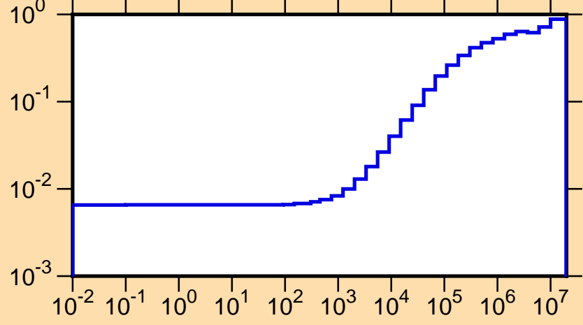
\mu vs. E for ^{114}\text{In}(\text{mt251})
