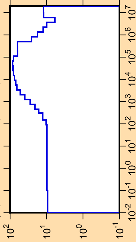
\Delta\mu/\mu vs. E for ^{114}\text{In}(\text{mt251})
