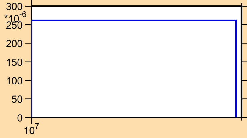
\sigma vs. E for ^{114}\text{In}(n,3n)
