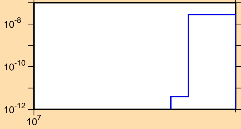
\sigma vs. E for ^{115}\text{In}(n,nt)
