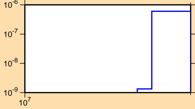
\sigma vs. E for ^{115}\text{In}(n,\text{nd})
