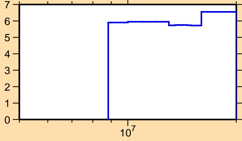
\Delta\sigma/\sigma vs. E for ^{115}\text{In}(n,\text{nonel.})
