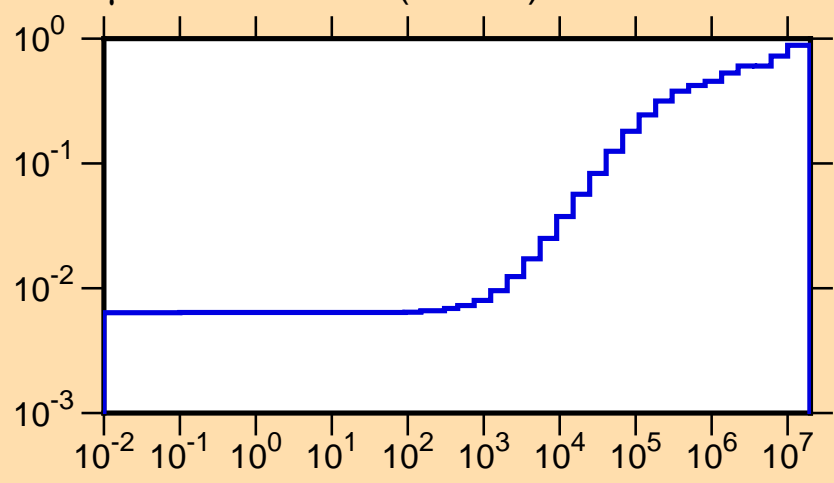
\mu vs. E for ^{115}\text{In}(\text{mt251})
