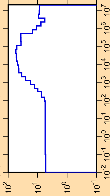
\Delta\mu/\mu vs. E for ^{115}\text{In}(\text{mt251})
