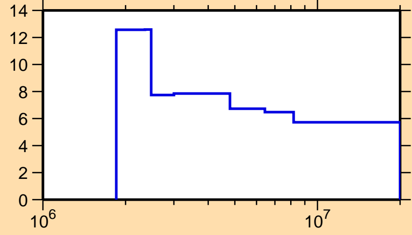
\Delta\sigma/\sigma vs. E for ^{115}\text{In}(n,n\text{nonel.})
