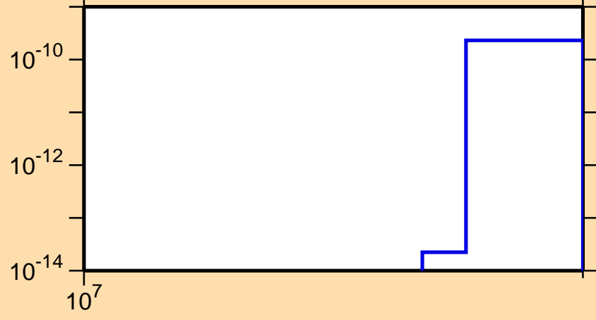
\sigma vs. E for ^{115}\text{In}(n,2n\alpha)
