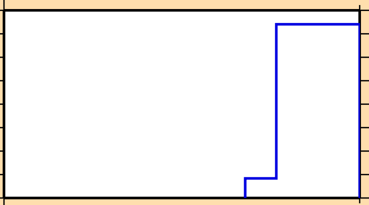
\sigma vs. E for ^{115}\text{In}(n,3n)
