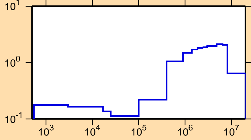
\sigma vs. E for ^{115}\text{In}(n,\text{inel.})
