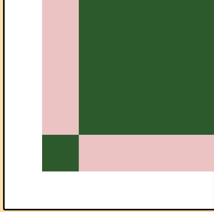
\sigma vs. E for ^{115}\text{In}(n,np)
