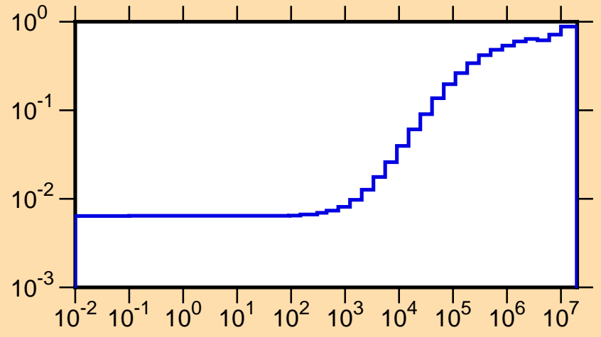
\mu vs. E for ^{116}\text{In}(\text{mt251})
