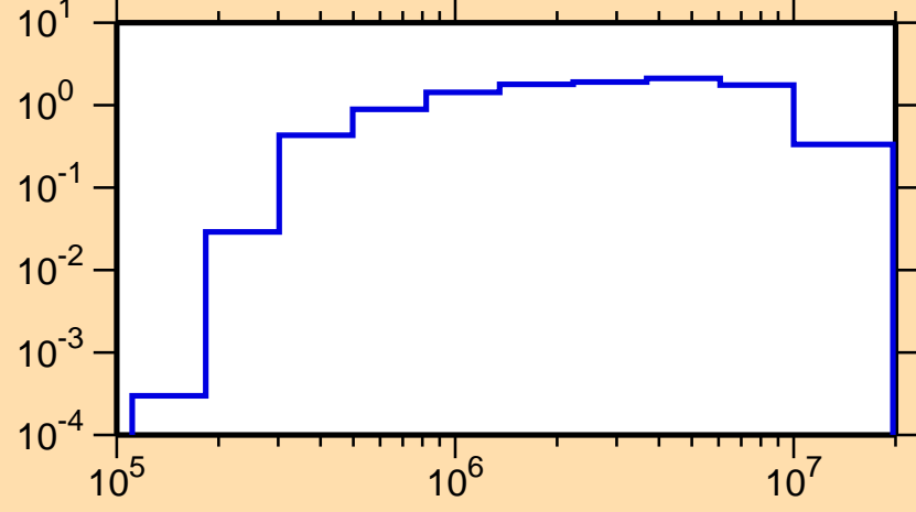
\sigma vs. E for ^{116}\text{In}(n,\text{inel.})
