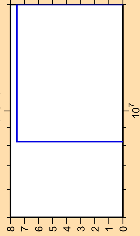
\Delta\sigma/\sigma vs. E for ^{116}\text{In}(n,p\alpha)
