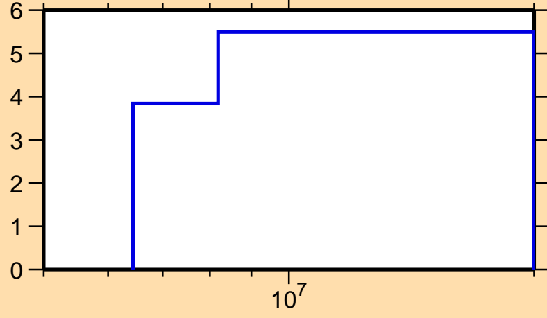
\Delta\sigma/\sigma vs. E for ^{116}\text{In}(n,\text{tot.})
