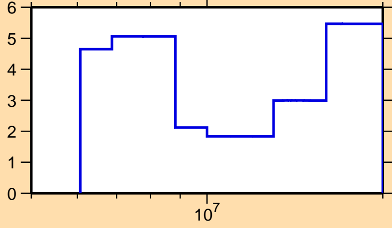
\Delta\sigma/\sigma vs. E for ^{116}\text{In}(n,\text{el.})
