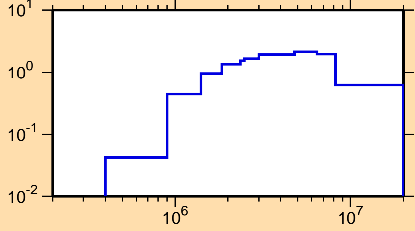
\sigma vs. E for ^{116}\text{In}(n,n\text{cont.})
