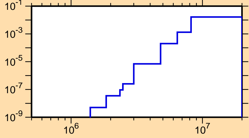
\sigma vs. E for ^{116}\text{In}(n,p)
