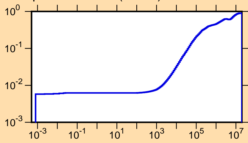
\mu vs. E for ^{117}\text{In}(\text{mt251})
