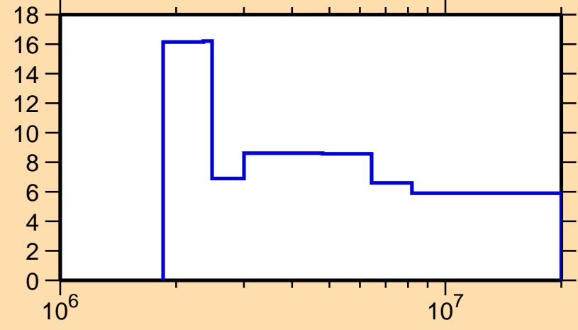
\Delta\sigma/\sigma vs. E for ^{117}\text{In}(n,n\text{nonel.})
