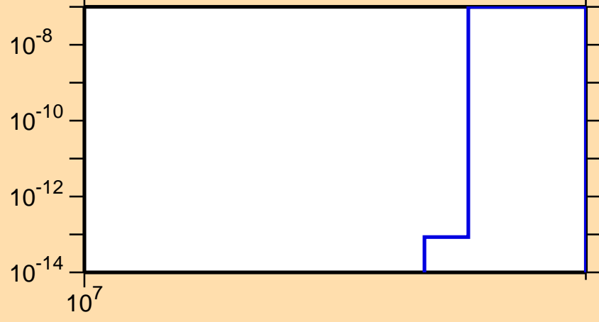
\sigma vs. E for ^{117}\text{In}(n,2np)
