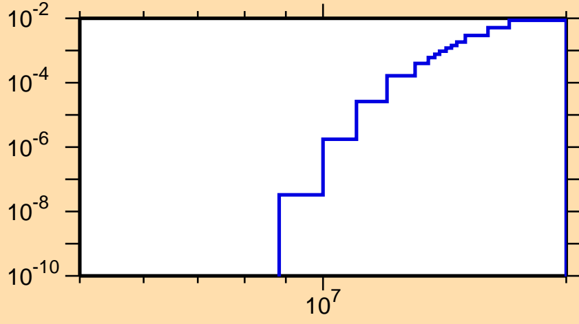
\sigma vs. E for ^{117}\text{In}(n,np)
