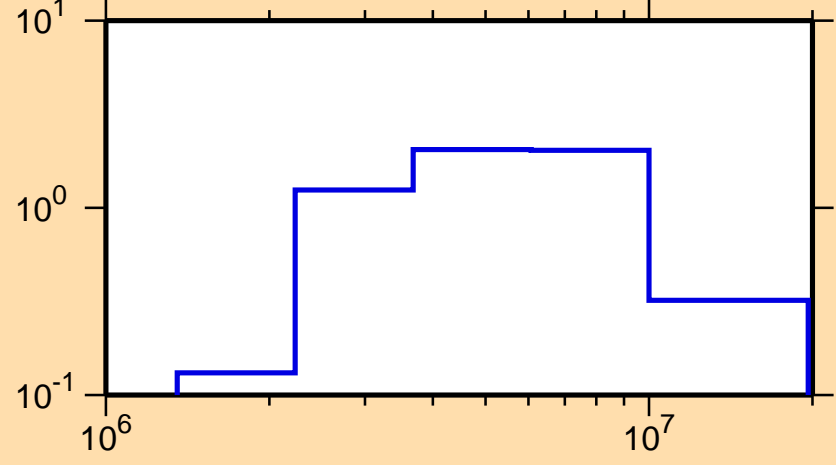
\sigma vs. E for ^{117}\text{In}(n,n\text{cont.})
