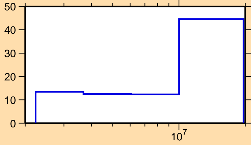
\Delta\sigma/\sigma vs. E for ^{117}\text{In}(n,ncont.)
