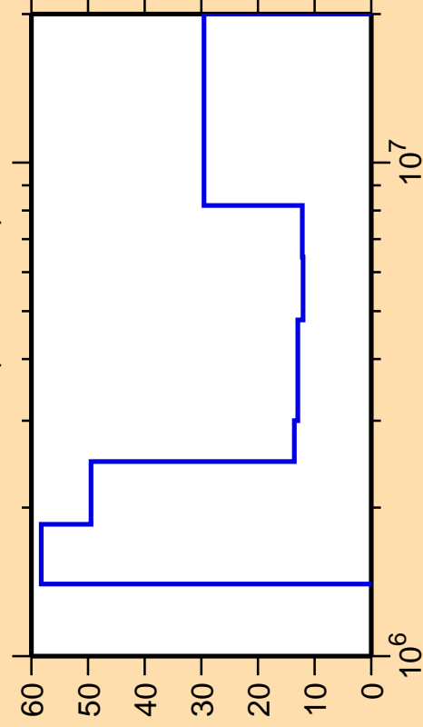
\Delta\sigma/\sigma vs. E for ^{117}\text{In}(n,\text{ncont.})
