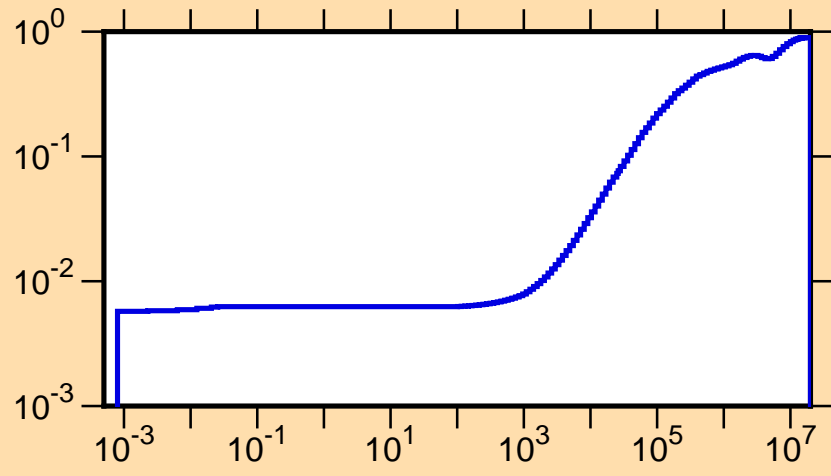
\mu vs. E for ^{118}\text{In}(\text{mt251})
