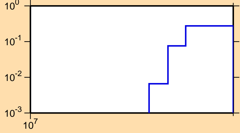
\sigma vs. E for ^{118}\text{In}(n,3n)
