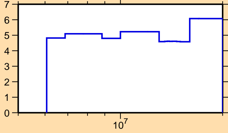
\Delta\sigma/\sigma vs. E for ^{118}\text{In}(n,\text{tot.})
