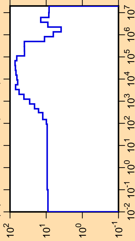
\Delta\mu/\mu vs. E for ^{118}\text{In}(\text{mt251})
