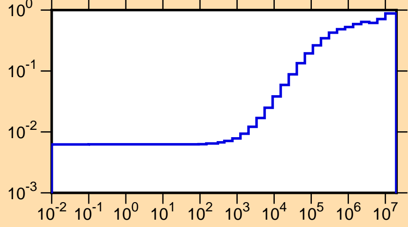
\mu vs. E for ^{118}\text{In}(\text{mt251})
