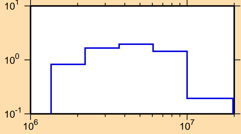
\sigma vs. E for ^{118}\text{In}(n,n\text{cont.})
