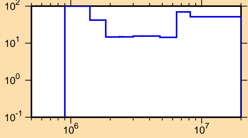
\Delta\sigma/\sigma vs. E for ^{118}\text{In}(n,n\text{cont.})
