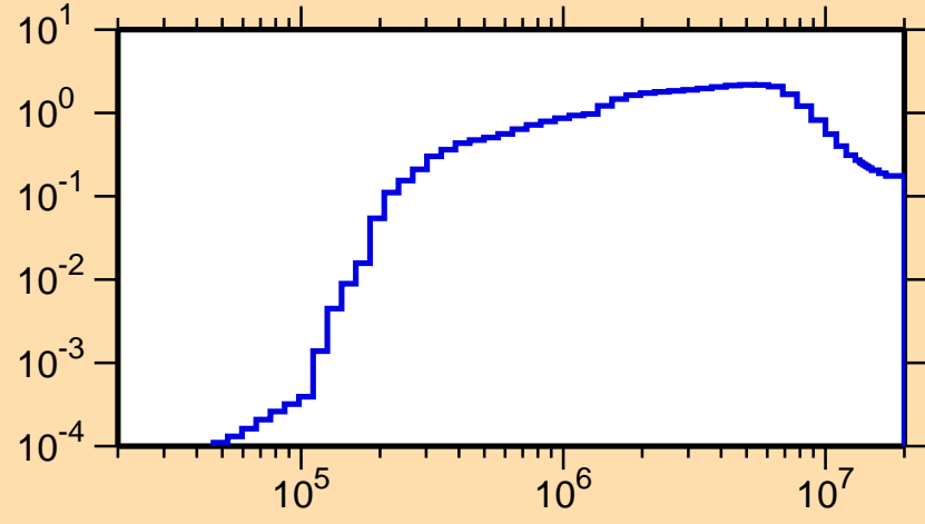
\sigma vs. E for ^{118}\text{In}(n,\text{inel.})
