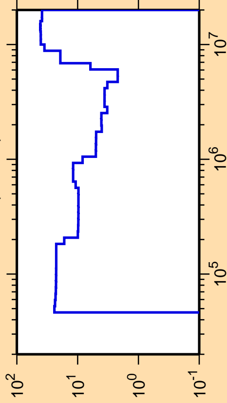
\Delta\sigma/\sigma vs. E for ^{118}\text{In}(n,\text{inel.})
