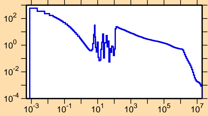
\sigma vs. E for ^{118}\text{In}(n,\gamma)
