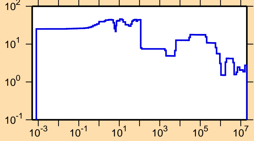
\Delta\sigma/\sigma vs. E for ^{118}\text{In}(n,\text{tot.})
