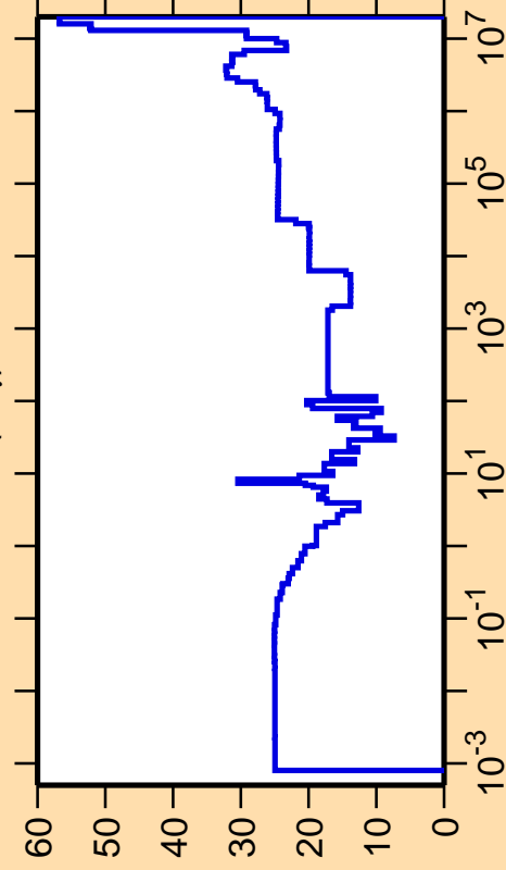
\Delta\sigma/\sigma vs. E for ^{118}\text{In}(n,\gamma)
