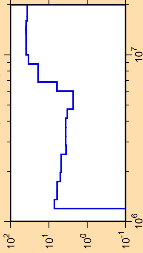
\Delta\sigma/\sigma vs. E for ^{118}\text{In}(n,\text{ncont.})
