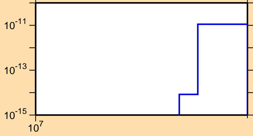
\sigma vs. E for ^{118}\text{In}(n,\text{He3})
