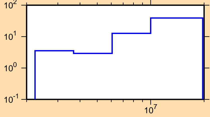
\Delta\sigma/\sigma vs. E for ^{118}\text{In}(n,ncont.)
