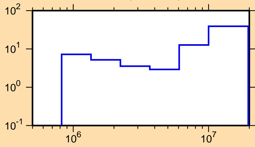
\Delta\sigma/\sigma vs. E for ^{118}\text{In}(n,ncont.)
