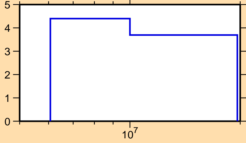
\Delta\sigma/\sigma vs. E for ^{118}\text{In}(n,\text{el.})
