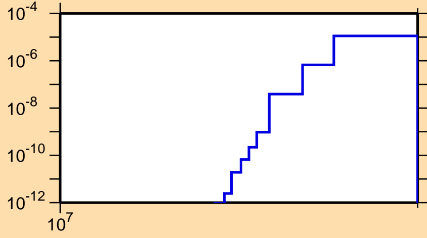
\sigma vs. E for ^{118}\text{In}(n,\text{nd})
