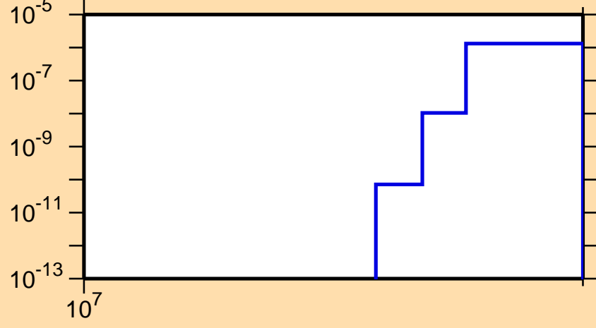
\sigma vs. E for ^{118}\text{In}(n,2np)
