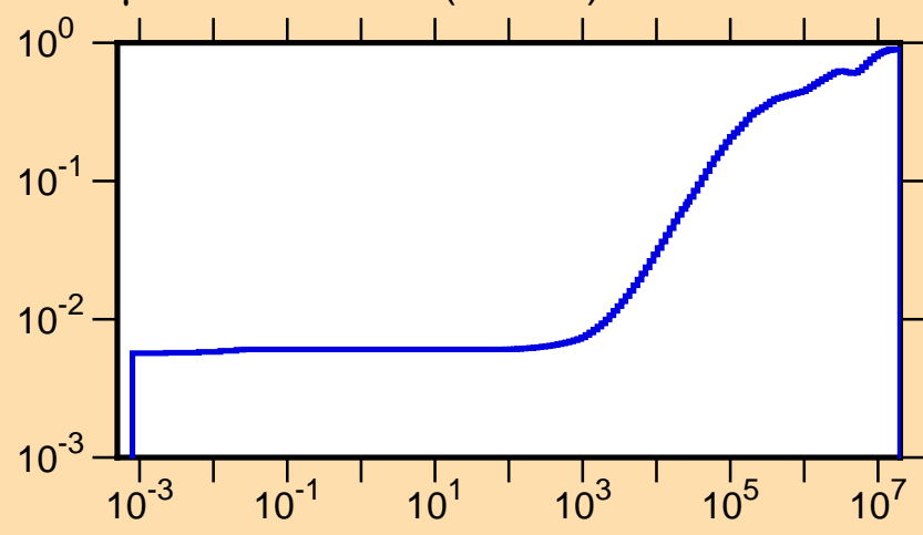
\mu vs. E for ^{119}\text{In}(\text{mt251})
