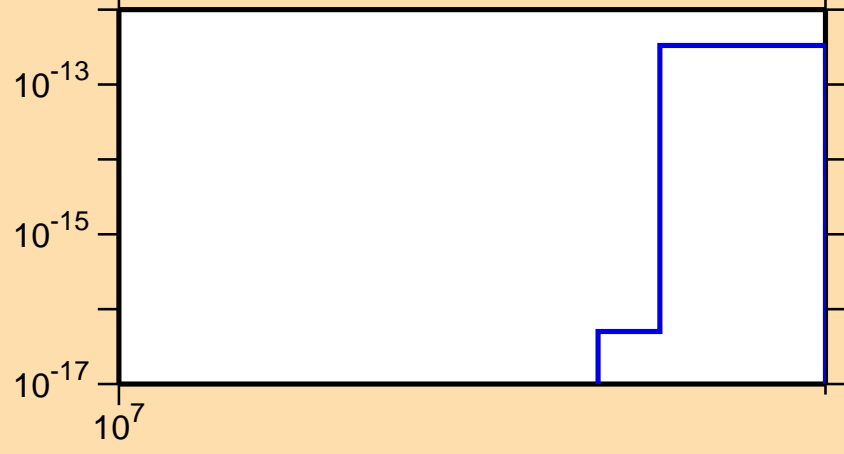
\sigma vs. E for ^{119}\text{In}(n,2n\alpha)
