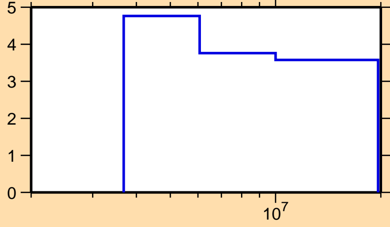
\Delta\sigma/\sigma vs. E for ^{119}\text{In}(n,\text{nonel.})
