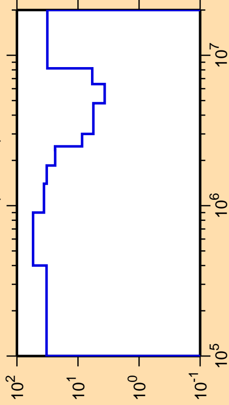
\Delta\sigma/\sigma vs. E for ^{119}\text{In}(n,\text{inel.})
