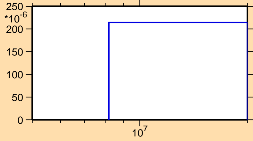
\sigma vs. E for ^{119}\text{In}(n,np)
