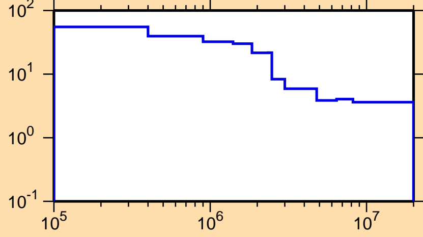
\Delta\sigma/\sigma vs. E for ^{119}\text{In}(n,\text{nonel.})
