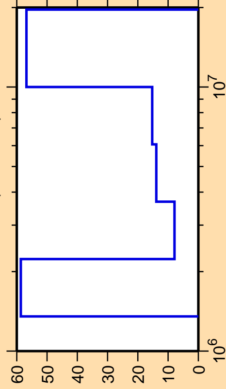
\Delta\sigma/\sigma vs. E for ^{119}\text{In}(n,\text{ncont.})
