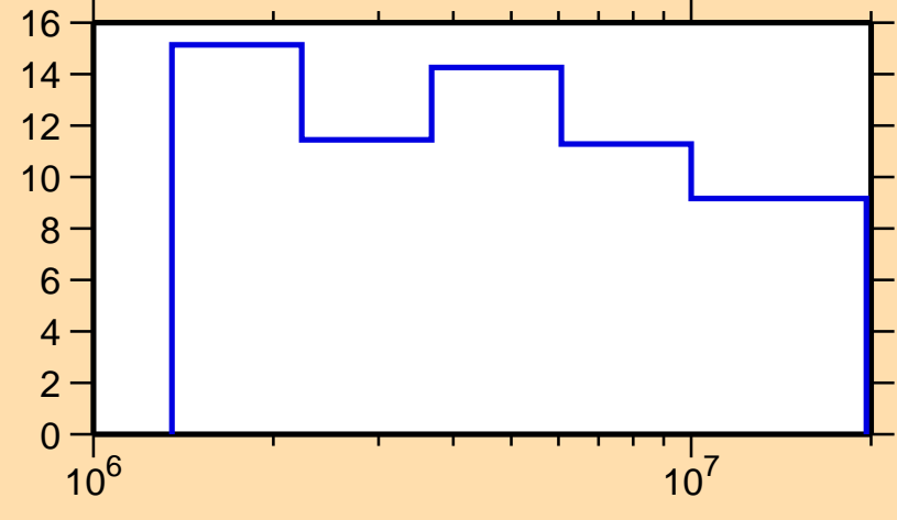
\Delta\sigma/\sigma vs. E for ^{119}\text{In}(n,n\text{nonel.})
