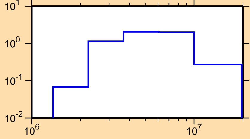
\sigma vs. E for ^{119}\text{In}(n,n\text{cont.})
