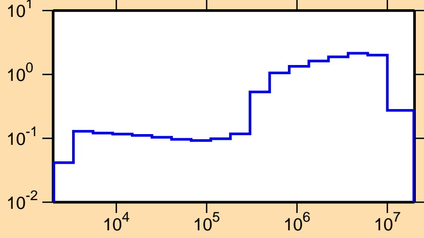
\sigma vs. E for ^{119}\text{In}(n,\text{inel.})
